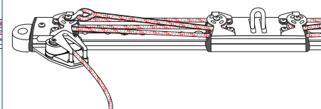
4:1 Traveller cleat on end
