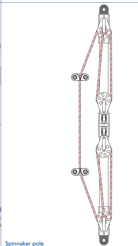
3:1 Remote cleat
