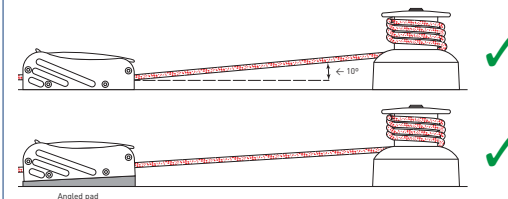
Clutch winch
