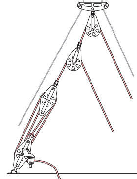
16:1 Split backstay
