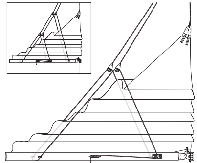
Lazy jacks
