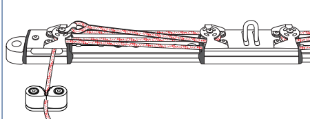
4:1 Remote cleats
