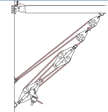
16:1 Cascaded kicker
