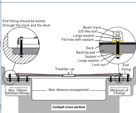
Beam track fitting
