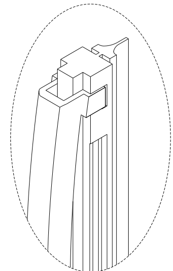
Figure – Blade Captive End
